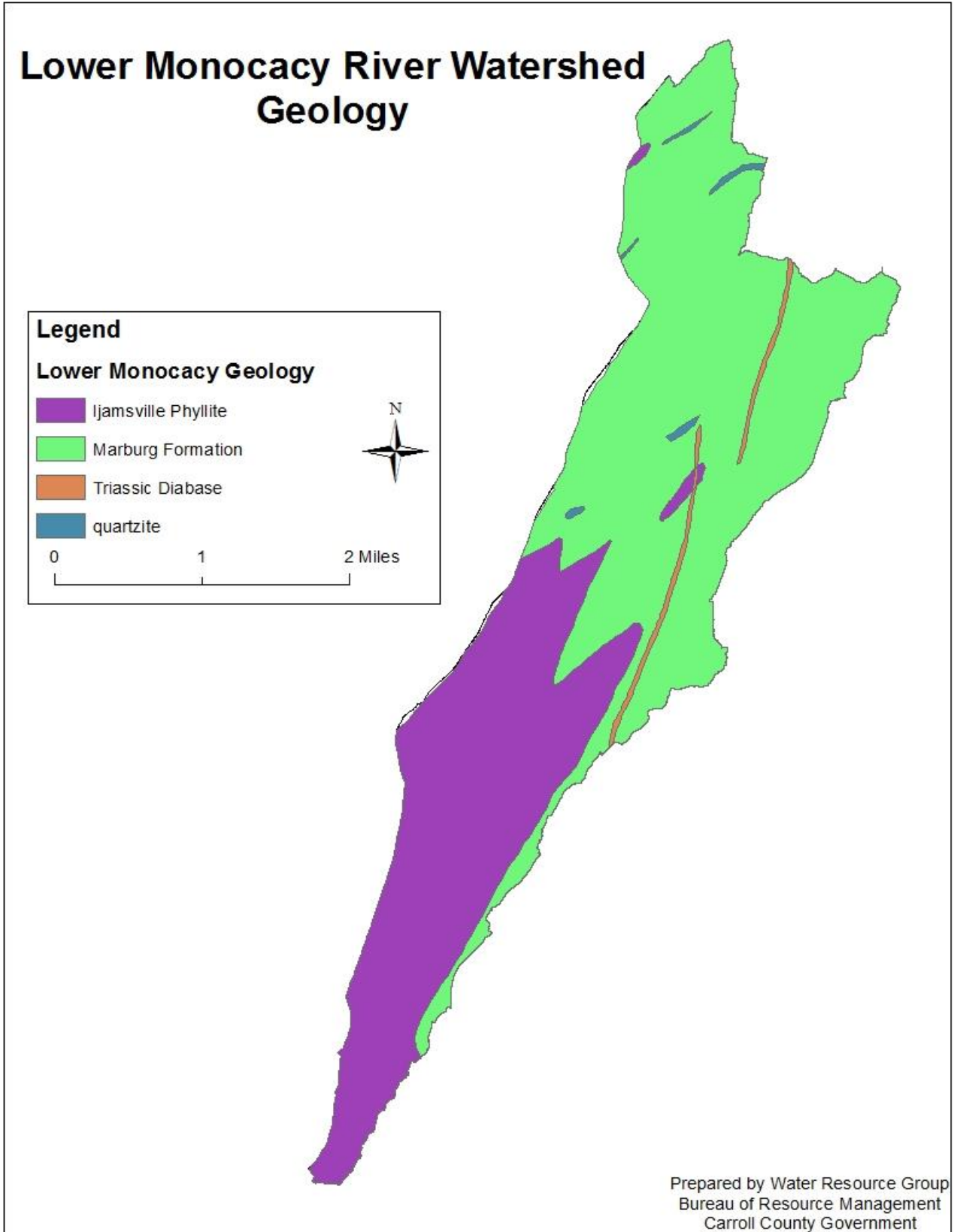
Figure 2-4: Lower Monocacy River Watershed Geology
