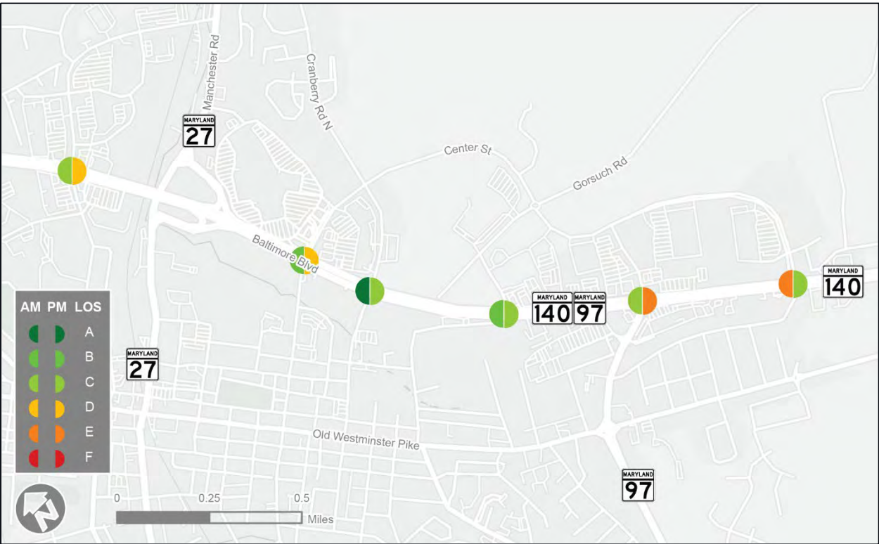
Figure 5.59 Westminster Existing Traffic Conditions
