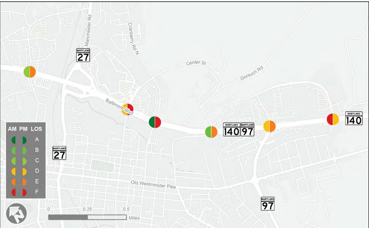
Figure 5.60 Westminster 2040 No-Build Traffic Conditions
