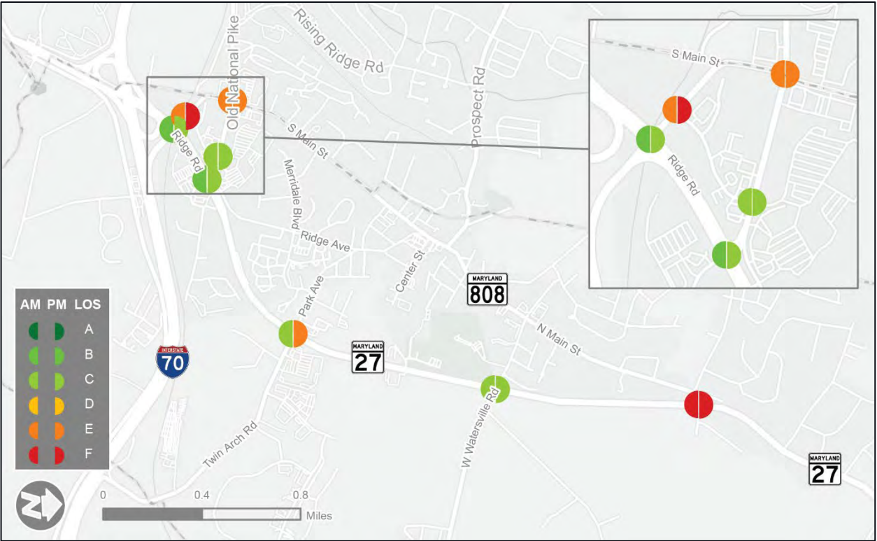
Figure 5.41 Mount Airy 2040 No-Build Traffic Conditions
