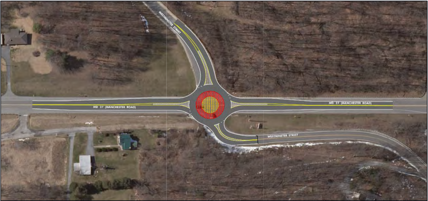
Figure 5.34 MD 27/Westminster Street Roundabout Concept
