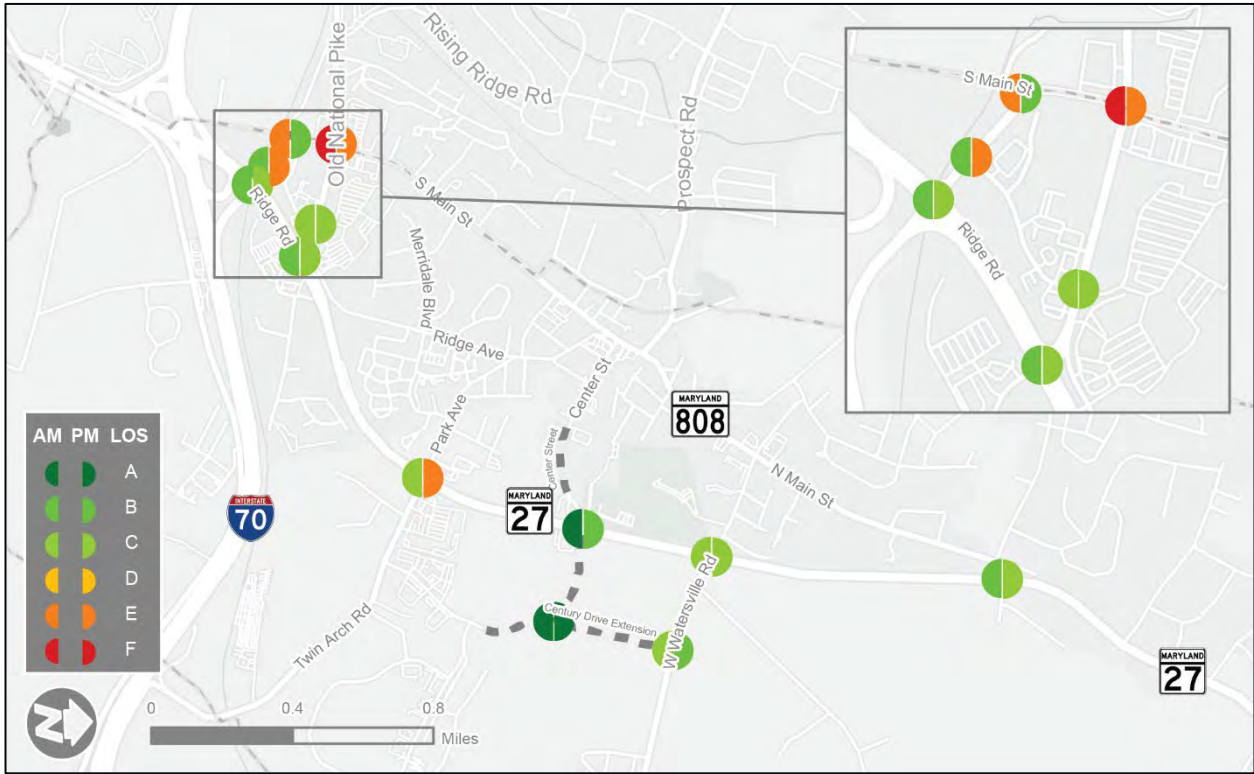
Figure 5.43 Mount Airy 2040 Build Traffic Conditions with Most Promising Potential Improvements
